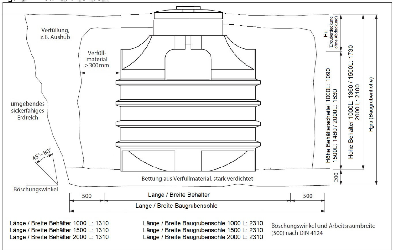
Figure 2: Installation sizes
